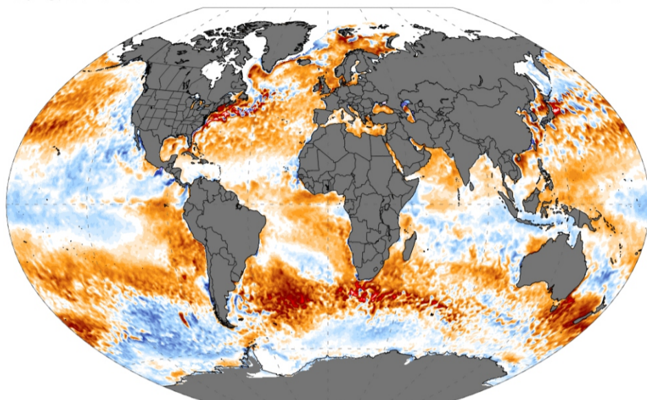
OISST SST Anomaly (°C) [1971-2000 baseline] 1-day Avg | Sun, Feb 19, 2023
